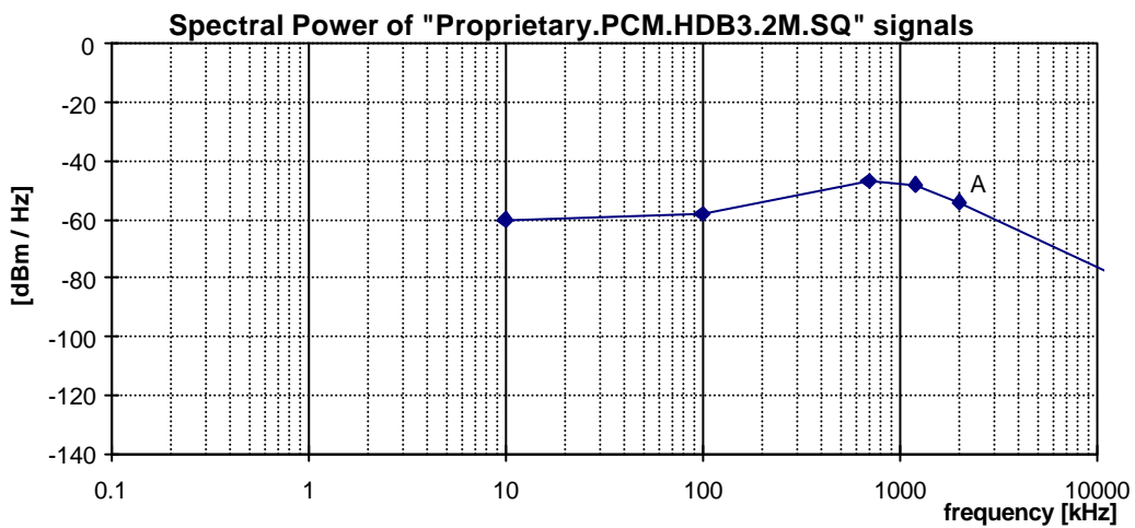
Figure 38: Spectral Power, for Proprietary.PCM.HDB3.2M.SQ signals, as specified in table 63
