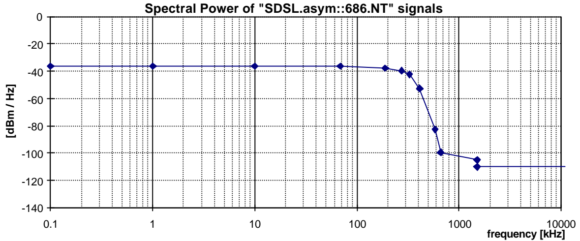
Figure 22: Spectral Power, for an "SDSL.asym::686.NT" signal, as specified in table 34
