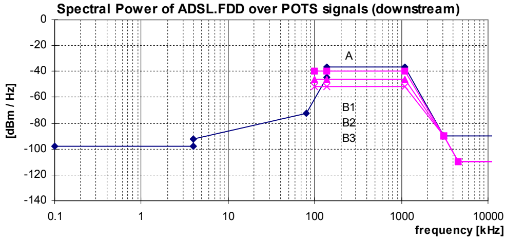
Figure 42: Spectral Power, for ADSL.FDD over POTS signals, as specified in table 69. The maximum spectral power varies with the value of parameter P_{BO} , as defined in table 70. Only the curves for the values P_{BO}=-40 dBm/Hz, P_{BO}=-46 dBm/Hz, and P_{BO}=-52 dBm/Hz are shown here
