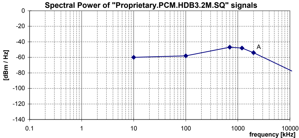
Figure 38: Spectral Power, for Proprietary.PCM.HDB3.2M.SQ signals, as specified in table 63
