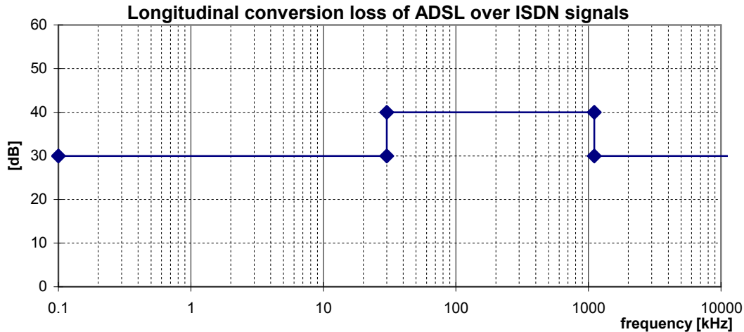
Figure 45: Minimum longitudinal conversion loss
