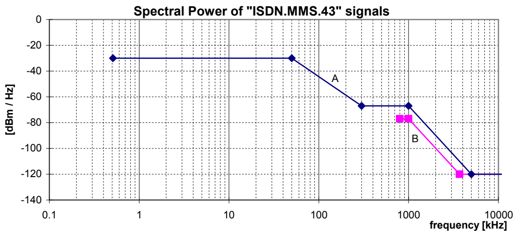
Figure 8: Spectral Power, for "ISDN.MMS.43" signals, as specified in table 10
