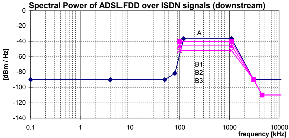
Figure 46: Spectral Power, for ADSL.FDD over ISDN signals, as specified in table 76. The maximum spectral power varies with the value of parameter P_{BO} , as defined in table 77. Only the curves for the values P_{BO} = -40 dBm/Hz, P_{BO} = -46 dBm/Hz, and P_{BO} = -52 dBm/Hz are shown here
