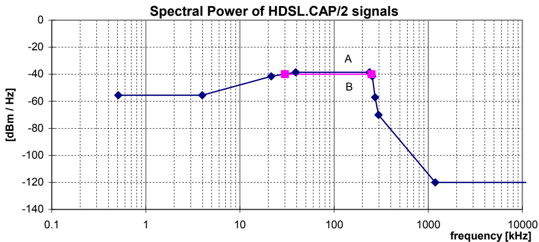
Figure 18: Spectral Power, for HDSL.CAP/2 signals, as specified in table 25
