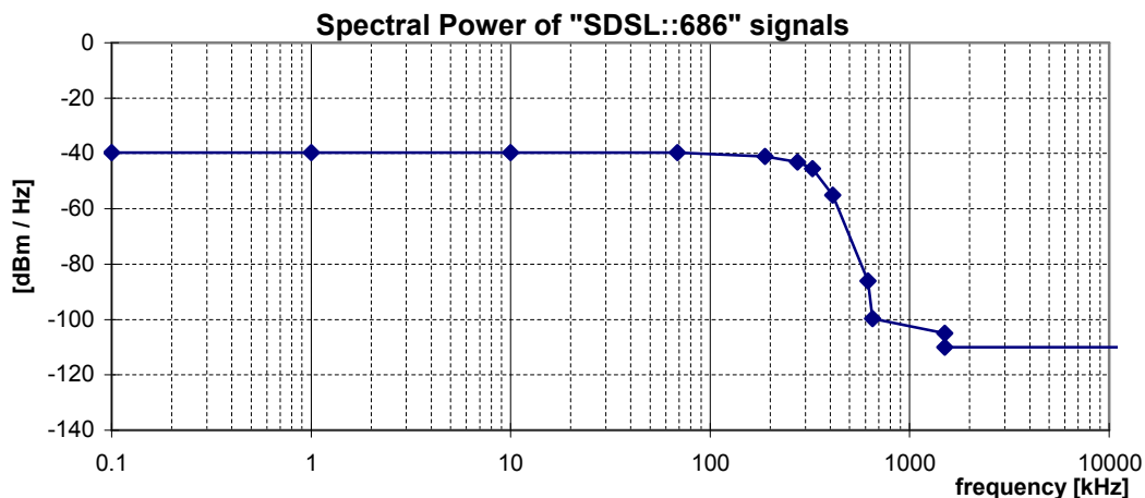
Figure 20: Spectral Power, for "SDSL::686" signals (at F_N=686 kHz), as specified in table 29. Note that these curves are dependent on the Principal frequency F_N , and that this figure shows an example only
