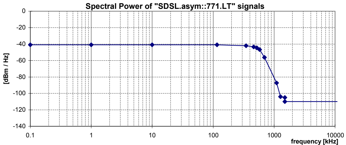
Figure 25: Spectral Power, for "SDSL.asym::771.LT" signal, as specified in table 36
