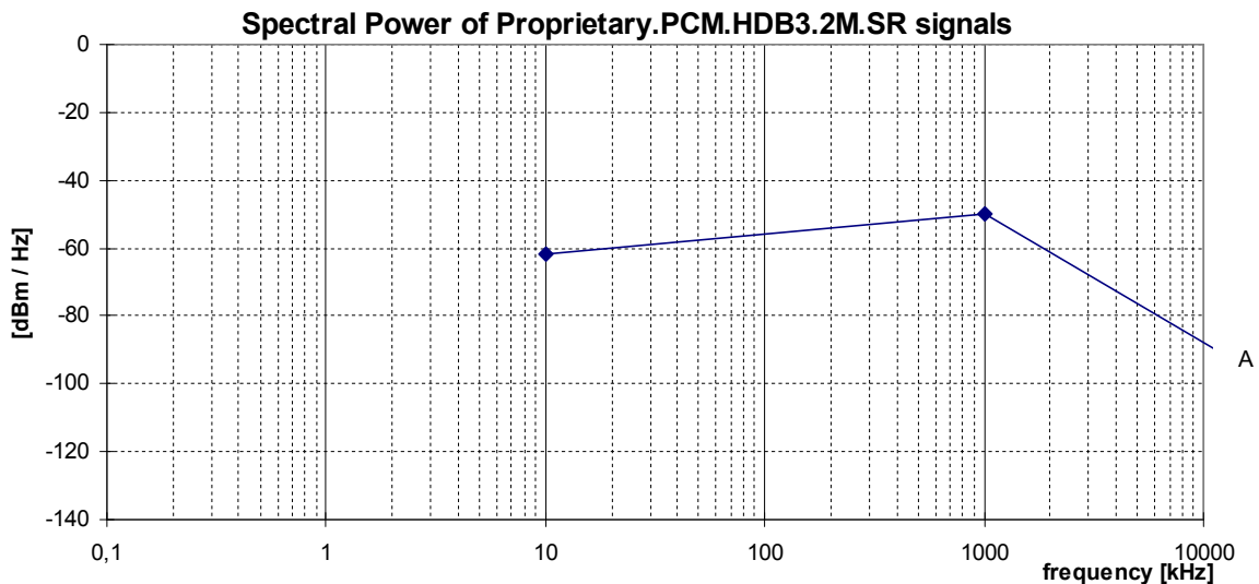
Figure 36: Spectral Power, for Proprietary.PCM.HDB3.2M.SR signals, as specified in table 60
