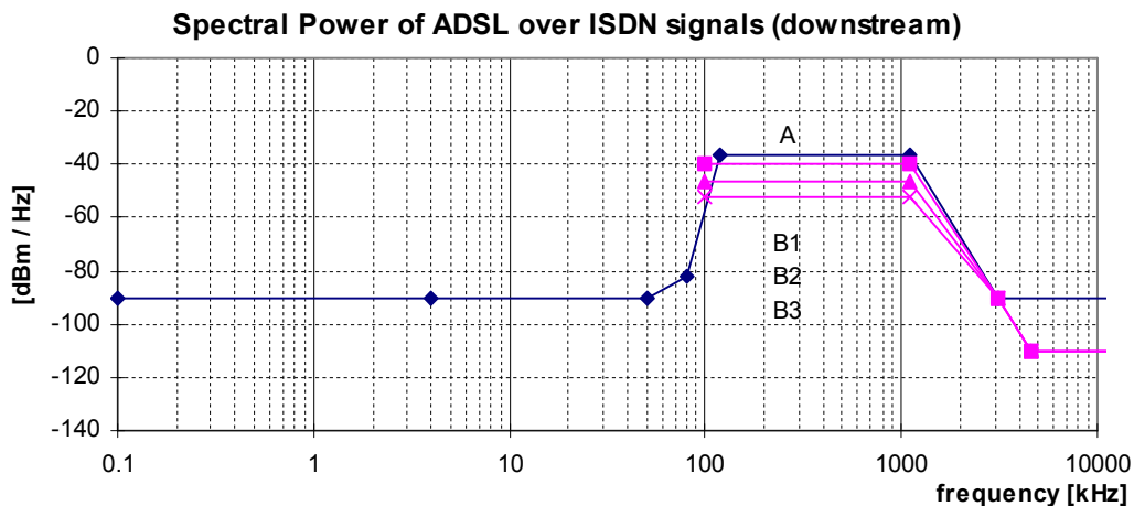
Figure 43: Spectral Power, for ADSL over ISDN signals, as specified in table 71. The maximum spectral power varies with the value of parameter P_{BO} , as defined in table 72. Only the curves for the values P_{BO} = -40 dBm/Hz, P_{BO} = -46 dBm/Hz, and P_{BO} = -52 dBm/Hz are shown here
