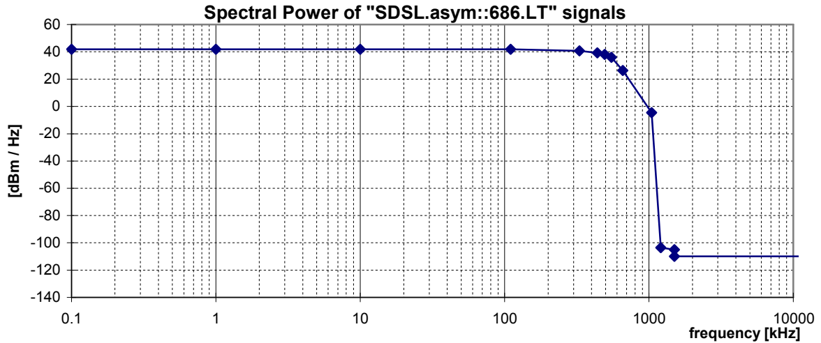
Figure 24: Spectral Power, for "SDSL.asym::686.LT" signal, as specified in table 36
