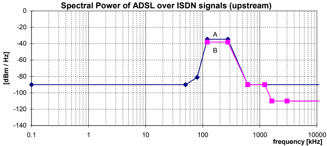
Figure 44: Spectral Power, for ADSL over ISDN signals, as specified in table 73
