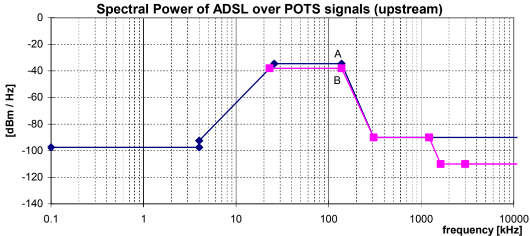
Figure 40: Spectral Power, for ADSL over POTS signals, as specified in table 66
