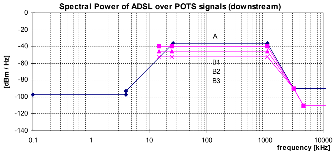
Figure 39: Spectral Power, for ADSL over POTS signals, as specified in table 64. The maximum spectral power varies with the value of parameter P_{BO} , as defined in table 65. Only the curves for the values P_{BO} = -40 dBm/Hz, P_{BO} = -46 dBm/Hz, and P_{BO} = -52 dBm/Hz are shown here
