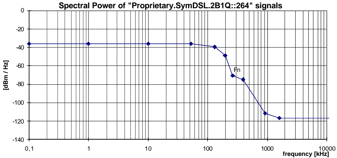
Figure 24: Spectral Power, for "Proprietary.SymDSL.2B1Q::264" signals (at F_N=264 kHz), as specified in Table 41. Note that these curves are dependent on the Principal frequency F_N , and that this figure shows an example only.
