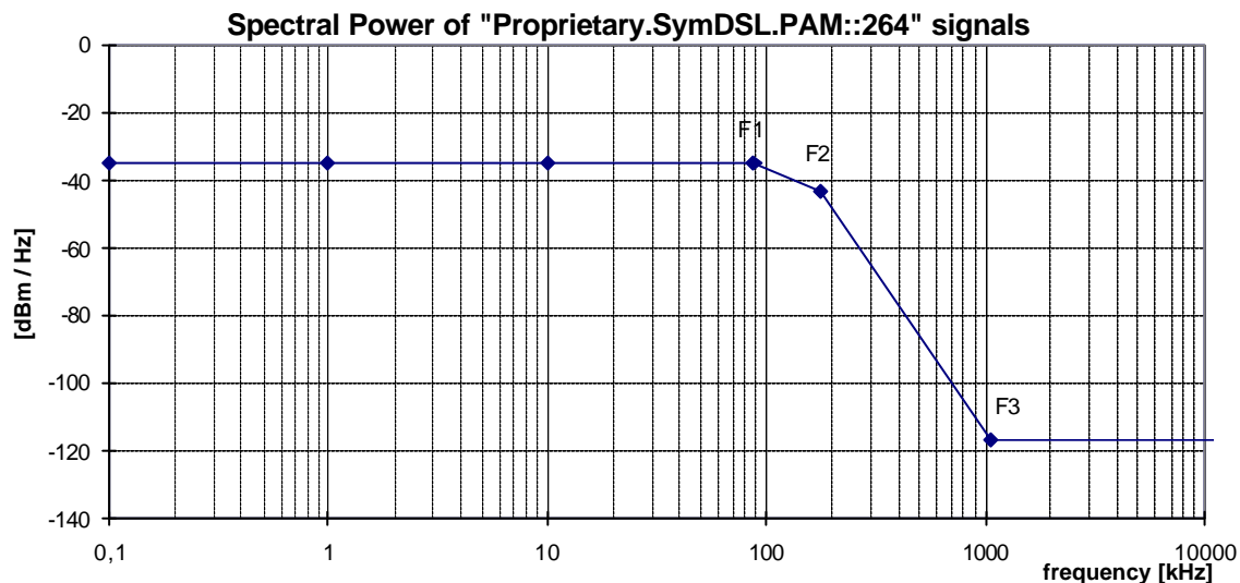
Figure 22: Spectral Power, for "Proprietary.SymDSL.PAM::264" signals (at F_N=264 kHz), as specified in table 41 and 42. Note that these curves are dependent on the Principal frequency F_N and that this figure shows an example only.
