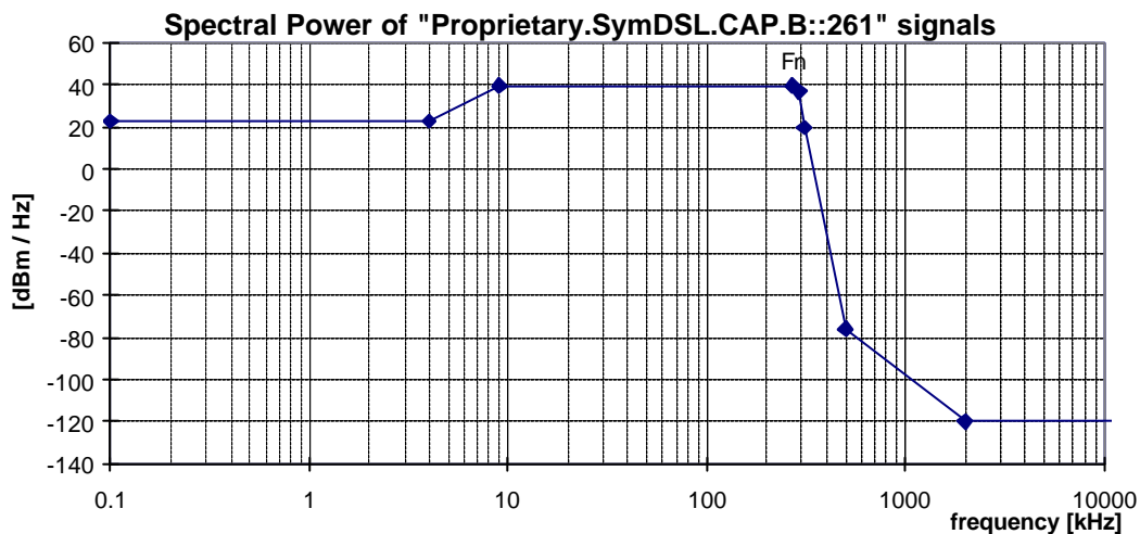
Figure 20: Spectral Power, for "Proprietary.SymDSL.CAP.B::261" signals (at F_N=261 kHz), as specified in table 37. Note that these curves are dependent on the Principal frequency F_N , and that this figure shows an example only.
