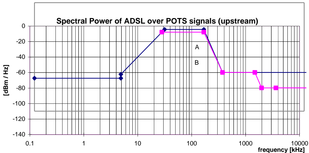
Figure 29: Spectral Power, for ADSL over POTS signals, as specified in table 58.
