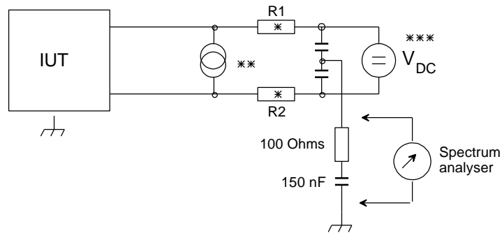
Figure 34: Measurement method for longitudinal output voltage (LOV).
