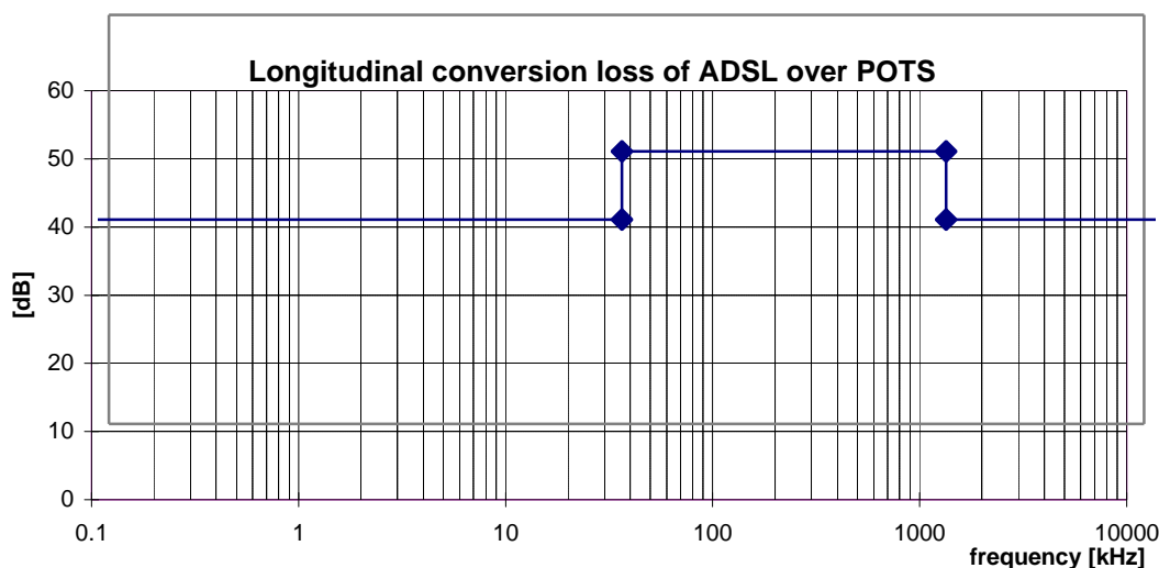
Figure 30: Minimum longitudinal conversion loss.
