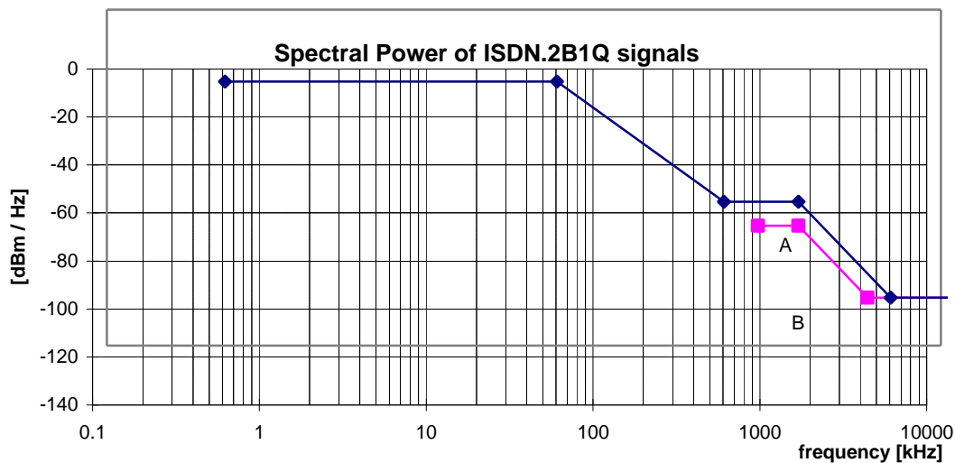
Figure 6: Spectral Power, for ISDN.2B1Q signals, as specified in table 8.
