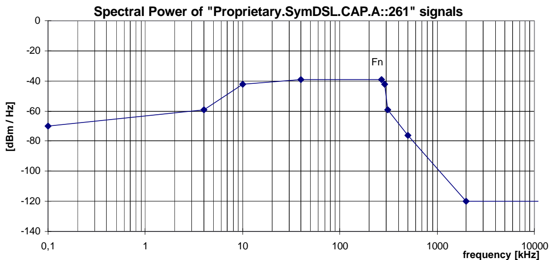
Figure 18: Spectral Power, for "Proprietary.SymDSL.CAP.A::261" signals (at F_N=261 kHz), as specified in table 33. Note that these curves are dependent on the Principal frequency F_N , and that this figure shows an example only.
