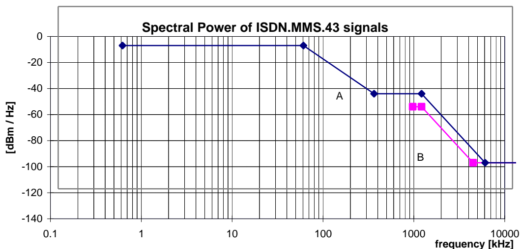
Figure 8: Spectral Power, for ISDN.MMS.43 signals, as specified in table 12.
