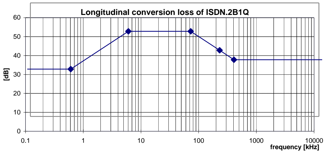
Figure 7: Minimum longitudinal conversion loss for a ISDN.2B1Q signal source
