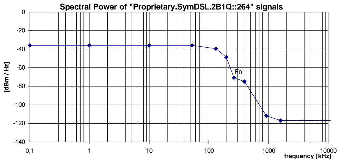
Figure 24: Spectral Power, for "Proprietary.SymDSL.2B1Q::264" signals (at F N =264 kHz), as specified in Table 41. Note that these curves are dependent on the Principal frequency F N , and that this figure shows an example only.
