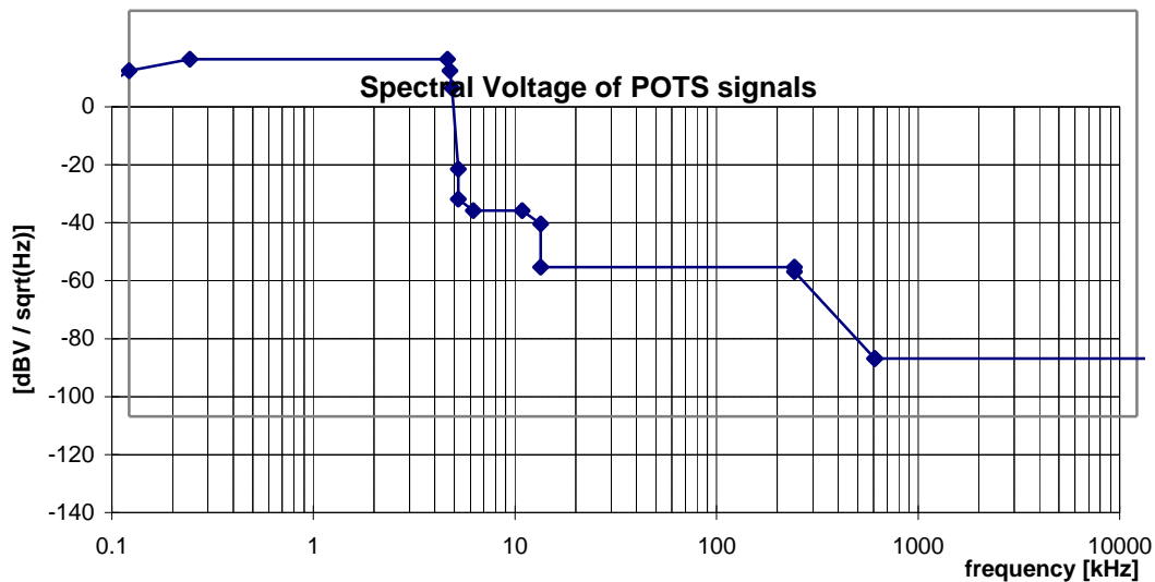
Figure 3: Spectral Voltage, for POTS signals, as specified in table 1.
