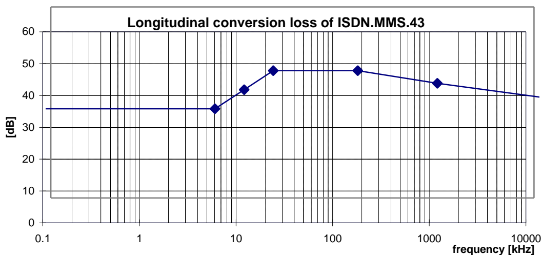
Figure 9: Minimum longitudinal conversion loss for a ISDN.MMS43 signal source
