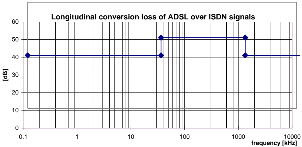
Figure 33: Minimum longitudinal conversion loss.
