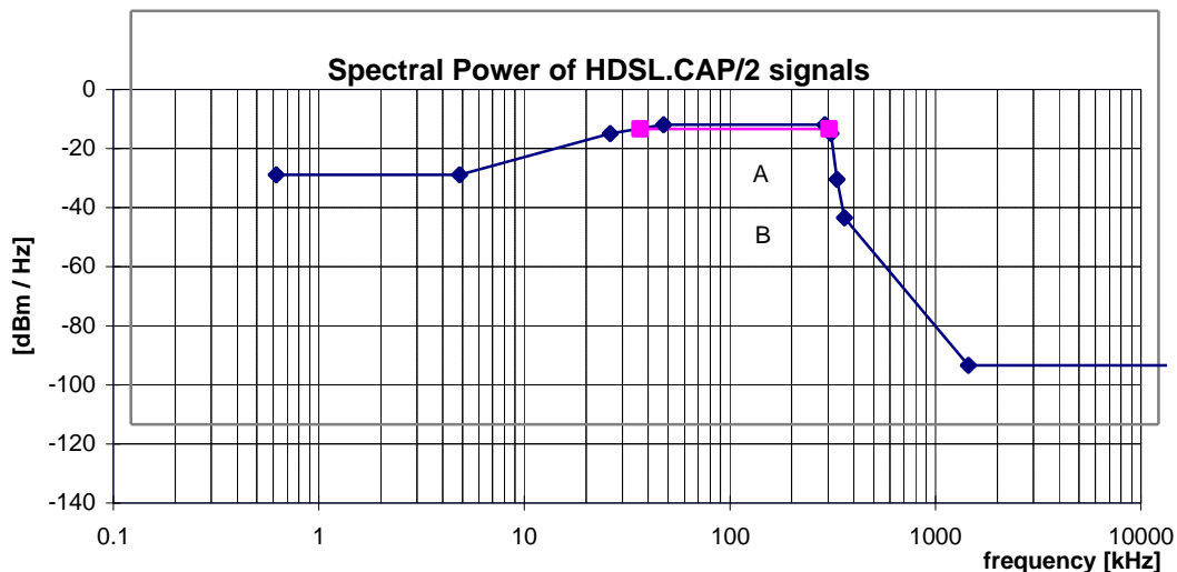
Figure 16: Spectral Power, for HDSL.CAP/2 signals, as specified in table 28.
