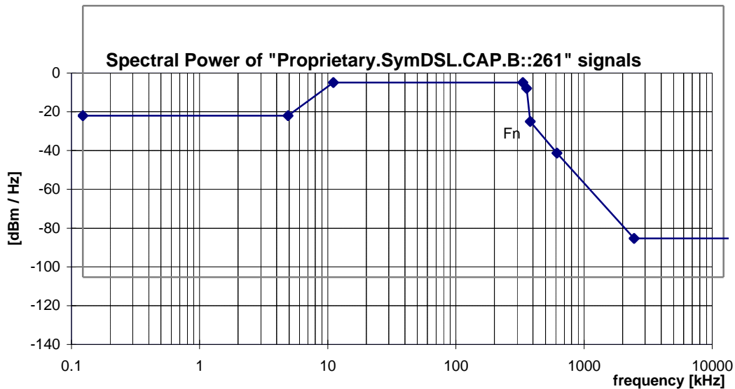
Figure 20: Spectral Power, for "Proprietary.SymDSL.CAP.B::261" signals (at F_N=261 kHz), as specified in table 37. Note that these curves are dependent on the Principal frequency F_N , and that this figure shows an example only.
