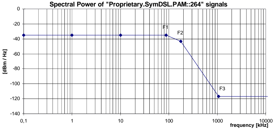
Figure 22: Spectral Power, for "Proprietary.SymDSL.PAM::264" signals (at F_N=264 kHz), as specified in table 41 and 42. Note that these curves are dependent on the Principal frequency F_N , and that this figure shows an example only.
