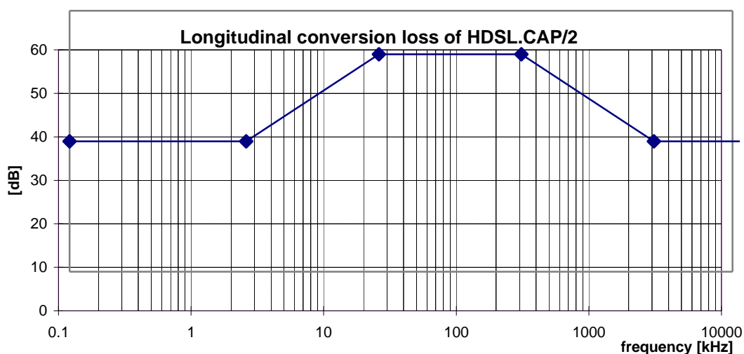
Figure 17: Minimum longitudinal conversion loss.
