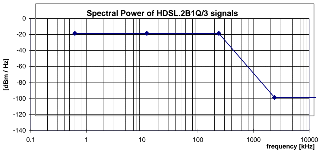
Figure 10: Spectral Power, for HDSL.2B1Q/3 signals, as specified in table 16.
