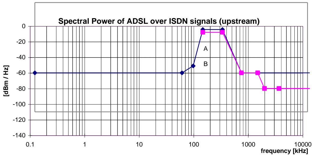
Figure 32: Spectral Power, for ADSL over ISDN signals, as specified in table 63.
