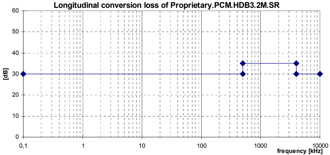
Figure 35: Minimum longitudinal conversion loss for a "Proprietary.PCM.HDB3.2M.SR" signal source
