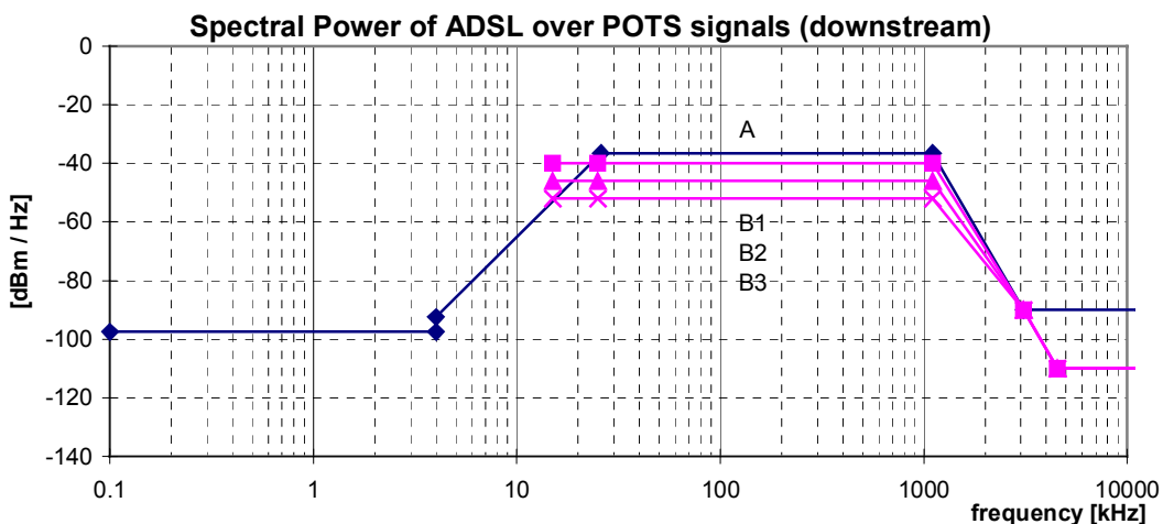
Figure 37: Spectral Power, for ADSL over POTS signals, as specified in table 71. The maximum spectral power varies with the value of parameter P_{BO} , as defined in table 72. Only the curves for the values P_{BO} = -40 dBm/Hz, P_{BO} = -46 dBm/Hz, and P_{BO} = -52 dBm/Hz are shown here
