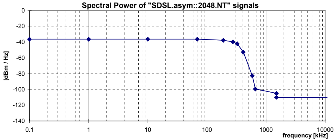
Figure 22: Spectral Power, for a "SDSL.asym::2048.NT" signal, as specified in Table 42.
