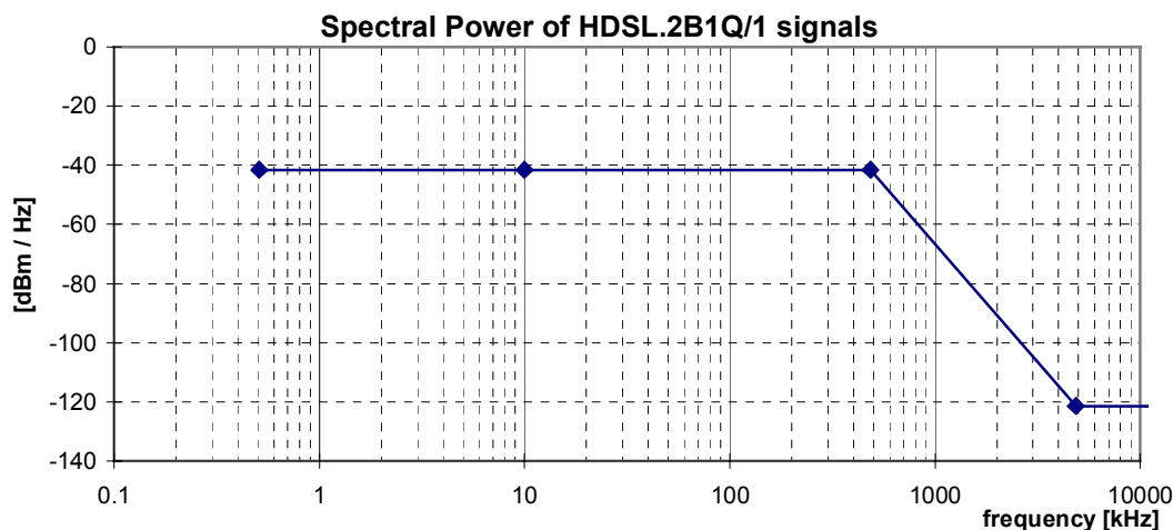
Figure 16: Spectral Power, for HDSL.2B1Q/1 signals, as specified in table 27
