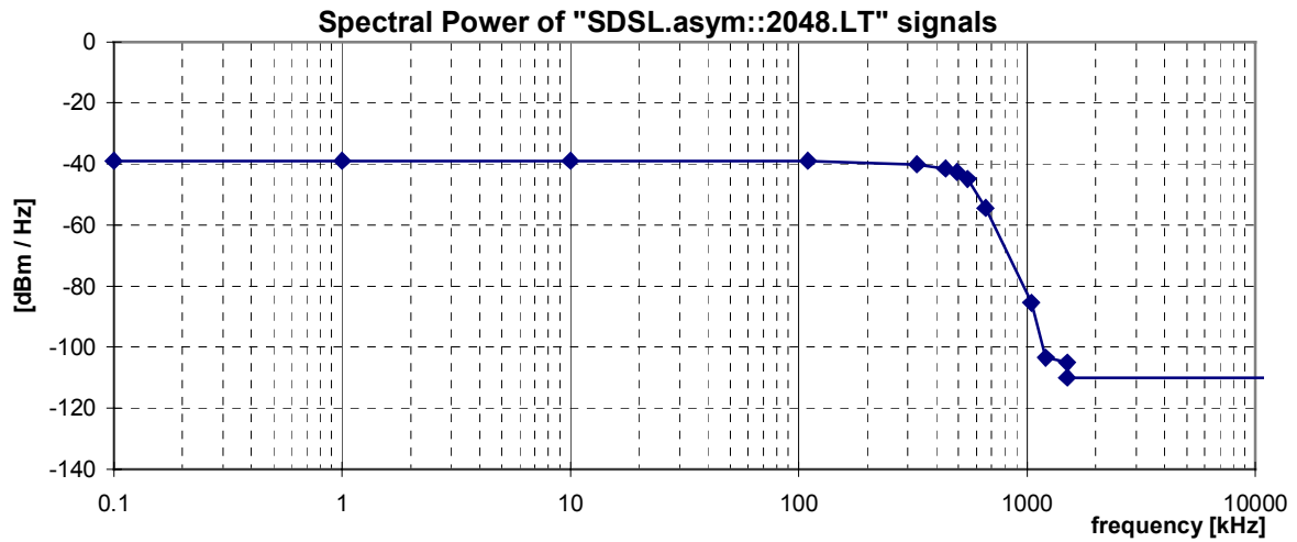
Figure 24: Spectral Power, for "SDSL.asym::2048.LT" signal, as specified in table 44.
