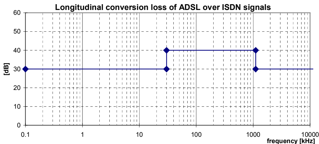
Figure 42: Minimum longitudinal conversion loss
