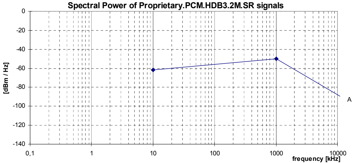
Figure 34: Spectral Power, for Proprietary.PCM.HDB3.2M.SR signals, as specified in table 66
