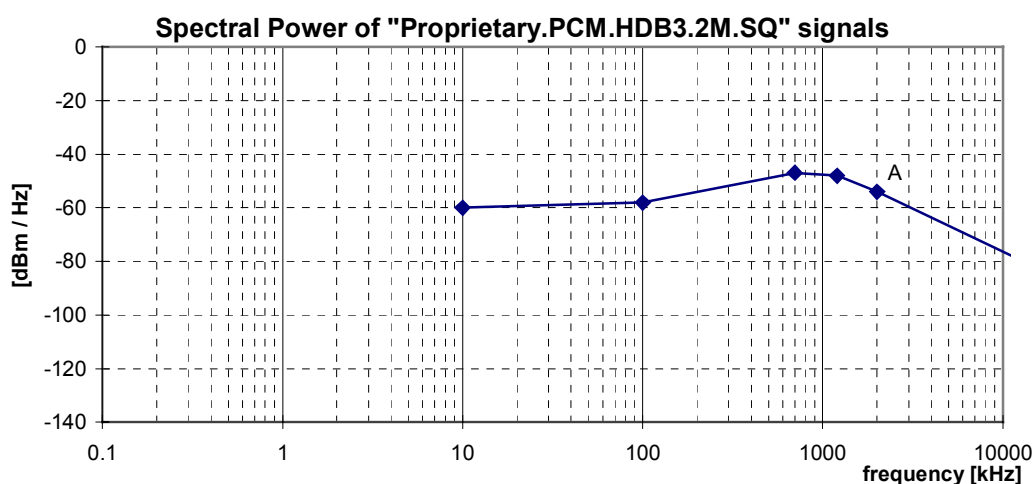
Figure 36: Spectral Power, for Proprietary.PCM.HDB3.2M.SQ signals, as specified in table 70
