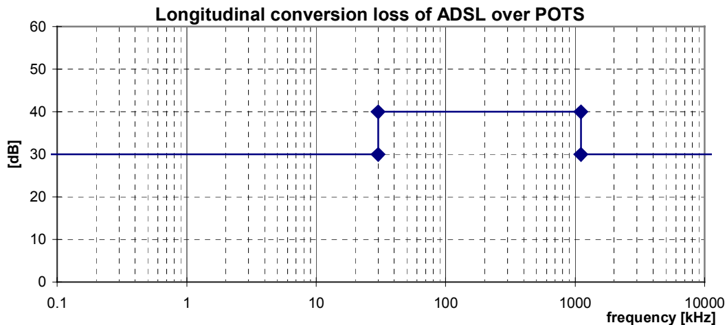
Figure 39: Minimum longitudinal conversion loss
