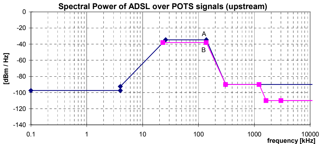
Figure 38: Spectral Power, for ADSL over POTS signals, as specified in table 73
