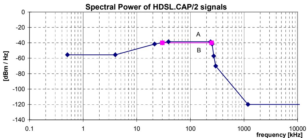
Figure 18: Spectral Power, for HDSL.CAP/2 signals, as specified in table 31
