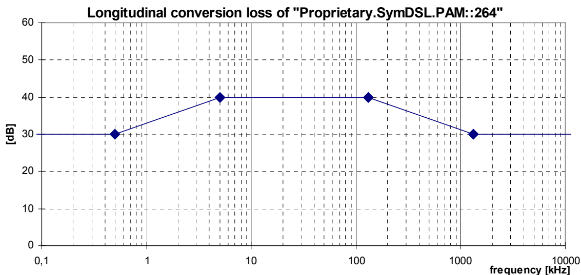
Figure 31: Minimum longitudinal conversion loss for a "Proprietary.SymDSL.PAM::264" signal source
