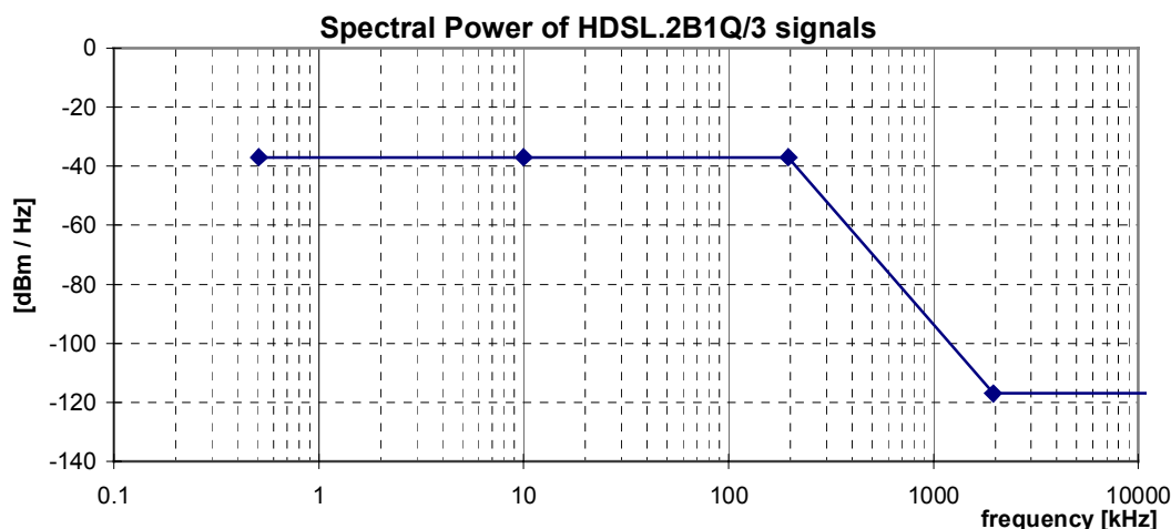
Figure 12: Spectral Power, for HDSL.2B1Q/3 signals, as specified in table 19
