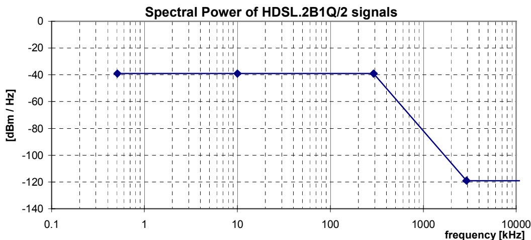
Figure 14: Spectral Power, for HDSL.2B1Q/2 signals, as specified in table 23
