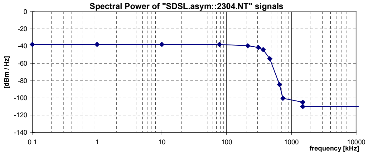
Figure 23: Spectral Power, for a "SDSL.asym::2304.NT" signal, as specified in Table 42.
