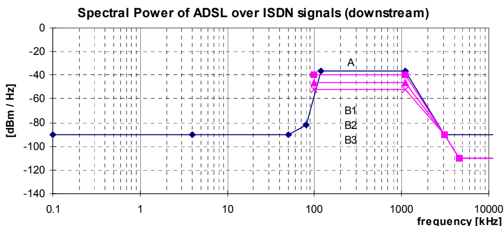
Figure 40: Spectral Power, for ADSL over ISDN signals, as specified in table 76. The maximum spectral power varies with the value of parameter P_{BO} , as defined in table 77. Only the curves for the values P_{BO} = -40 dBm/Hz, P_{BO} = -46 dBm/Hz, and P_{BO} = -52 dBm/Hz are shown here
