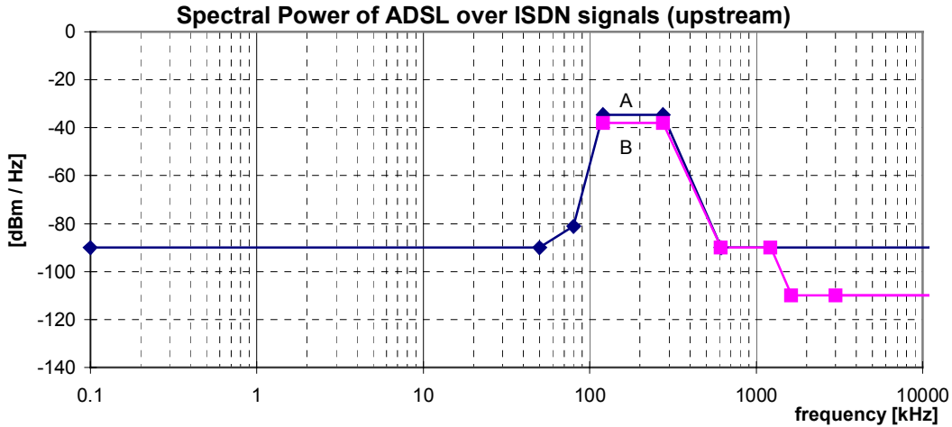
Figure 41: Spectral Power, for ADSL over ISDN signals, as specified in table 78
