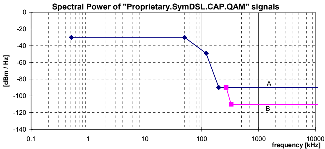
Figure 10: Spectral Power, for "Proprietary.SymDSL.CAP.QAM" signals, as specified in table 16.
