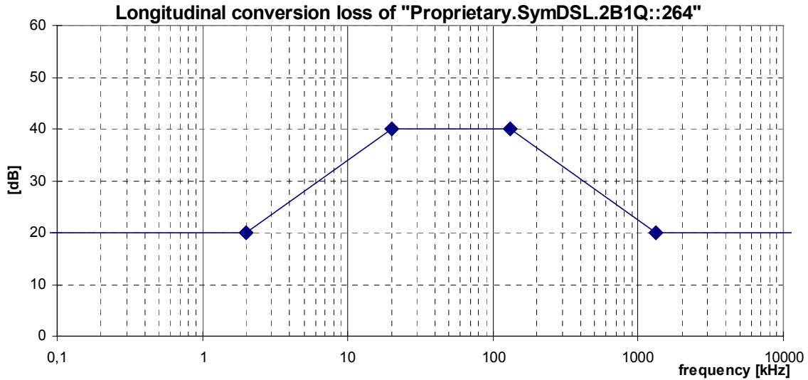
Figure 33: Minimum longitudinal conversion loss for a "Proprietary.SymDSL.2B1Q::264" signal source
