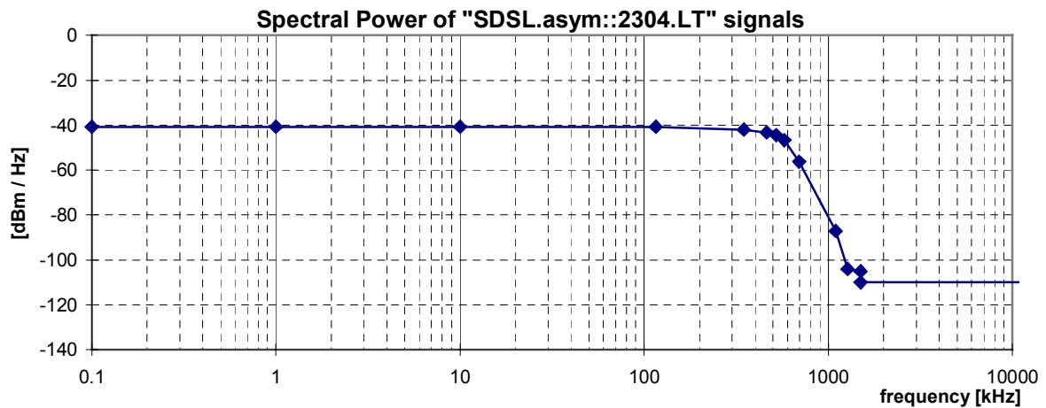
Figure 25: Spectral Power, for "SDSL.asym::2304.LT" signal, as specified in table 44.
