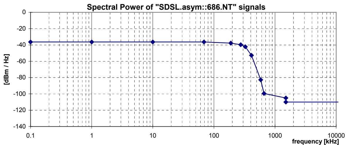
Figure 22: Spectral Power, for a "SDSL.asym::686.NT" signal, as specified in Table 43.
