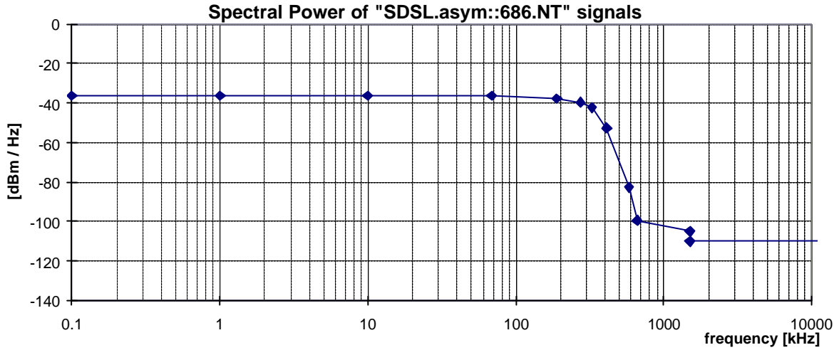
Figure 22: Spectral Power, for an "SDSL.asym::686.NT" signal, as specified in table 34
