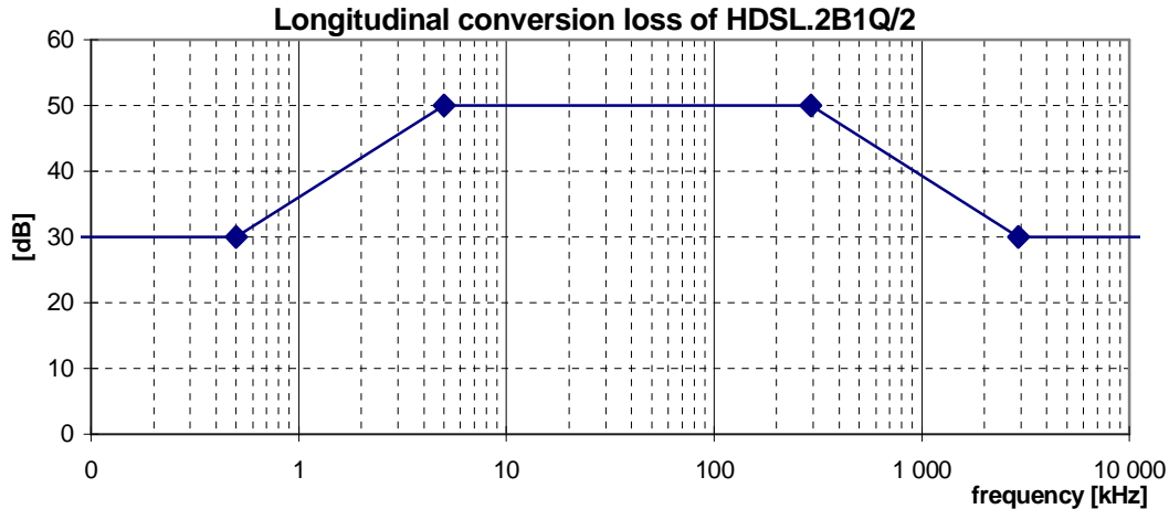
Figure 15: Minimum longitudinal conversion loss for a HDSL.2B1Q/2 signal source (584 kbaud/wirepair)
