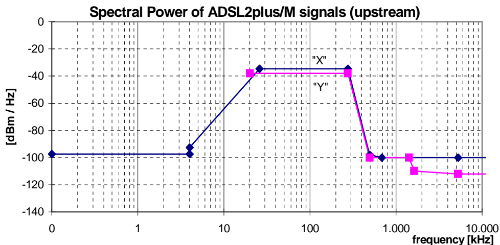
Figure 59: Spectral Power, for upstream ADSL2plus/M signals, as specified in table 93.
