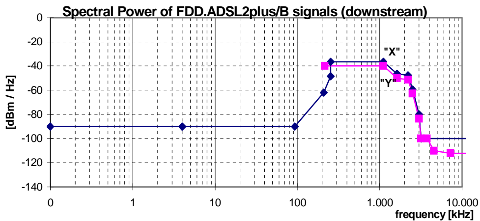
Figure 54: Spectral Power, for downstream FDD.ADSL2plus/B signals, specified in table 89.
