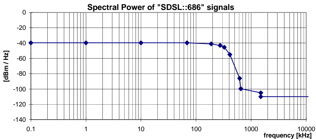
Figure 20: Spectral Power, for "SDSL::686" signals (at F_N=686 kHz), as specified in table 36. Note that these curves are dependent on the Principal frequency F_N , and that this figure shows an example only
