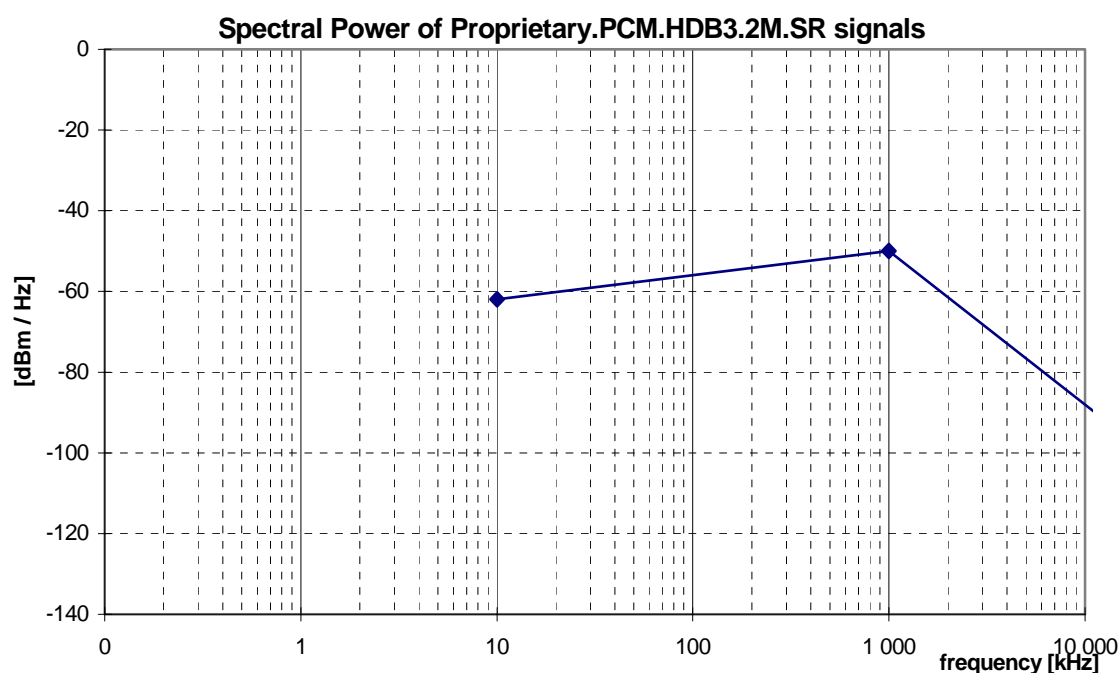
Figure 36: Spectral Power, for Proprietary.PCM.HDB3.2M.SR signals, as specified in table 60
