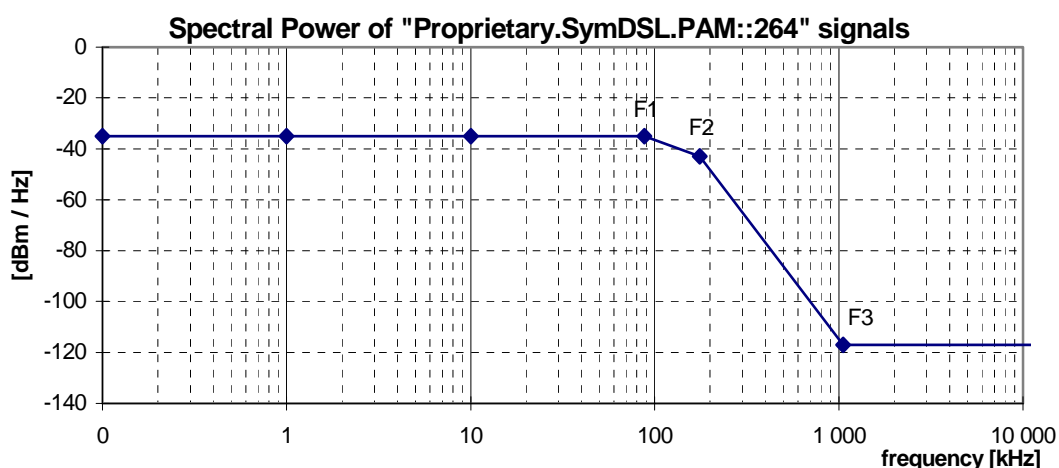
Figure 32: Spectral Power, for "Proprietary.SymDSL.PAM::264" signals (at F_N = 264 kHz), as specified in tables 51 and 52
