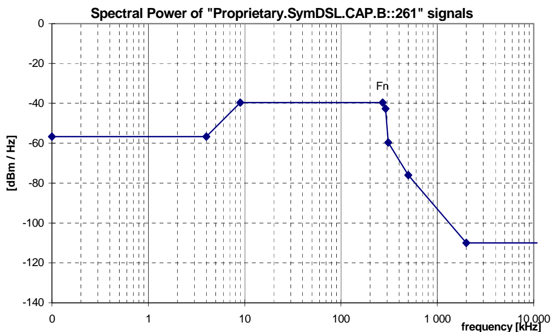
Figure 28: Spectral Power, for "Proprietary.SymDSL.CAP.B::261" signals (at F_N = 261 kHz), as specified in table 43
