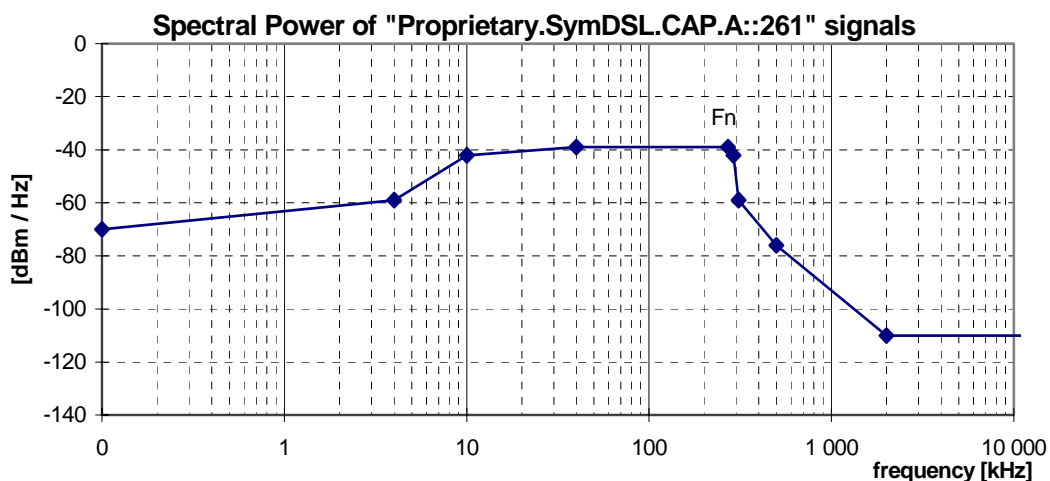
Figure 26: Spectral Power, for "Proprietary.SymDSL.CAP.A::261" signals (at F_N = 261 kHz), as specified in table 39
