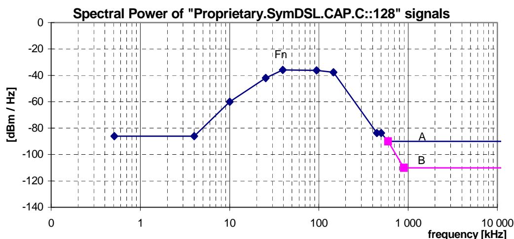
Figure 30: Spectral Power, for "Proprietary.SymDSL.CAP.C::128" signals (at F_N = 128 \text{ kHz} ), as specified in table 47
