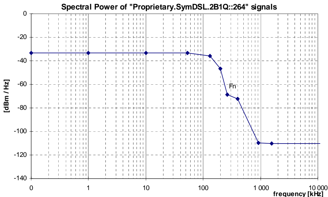
Figure 34: Spectral Power, for "Proprietary.SymDSL.2B1Q::264" signals (at F_N = 264 kHz), as specified in table 51
