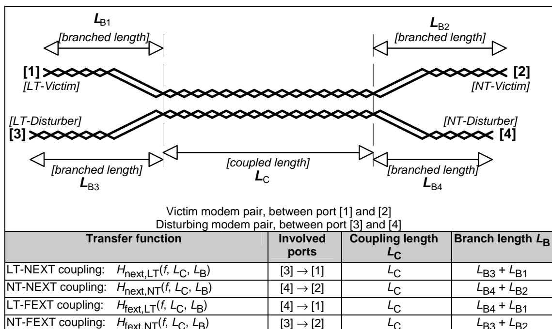
Figure 12: Example of the lengths that are to be used for evaluating branched normalized NEXT and FEXT
